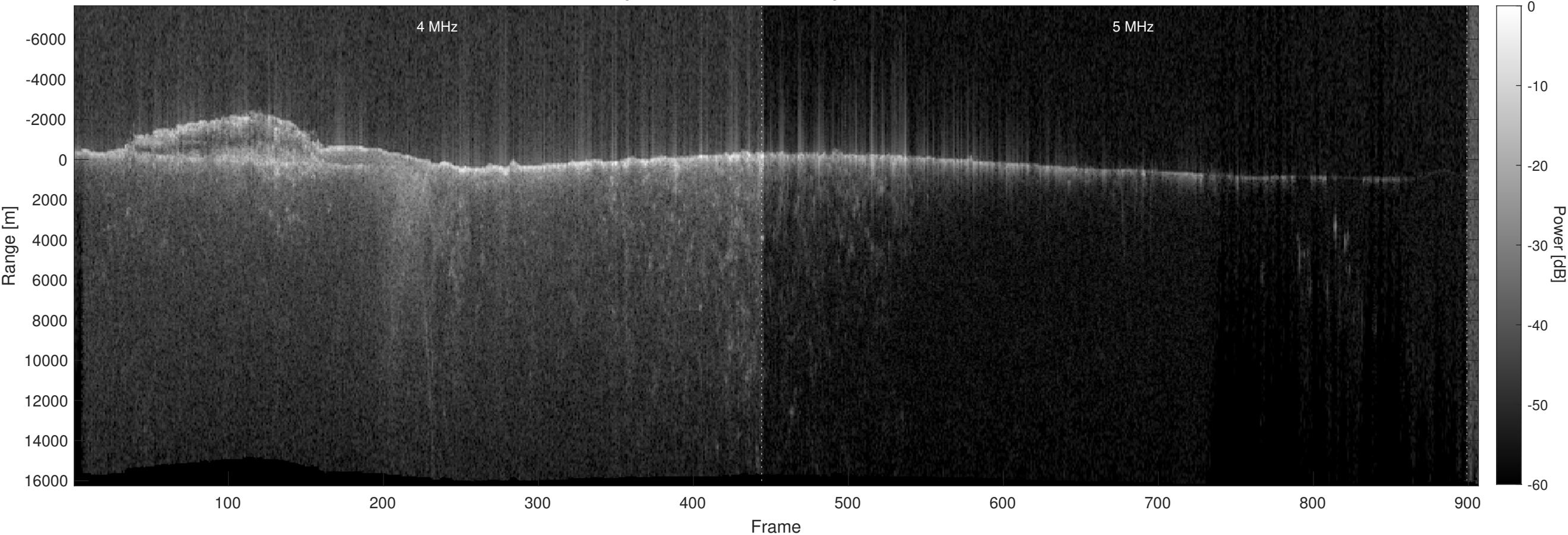
Orbit 11651, Optimized, No Window, Depth-Corrected, Channel 2
