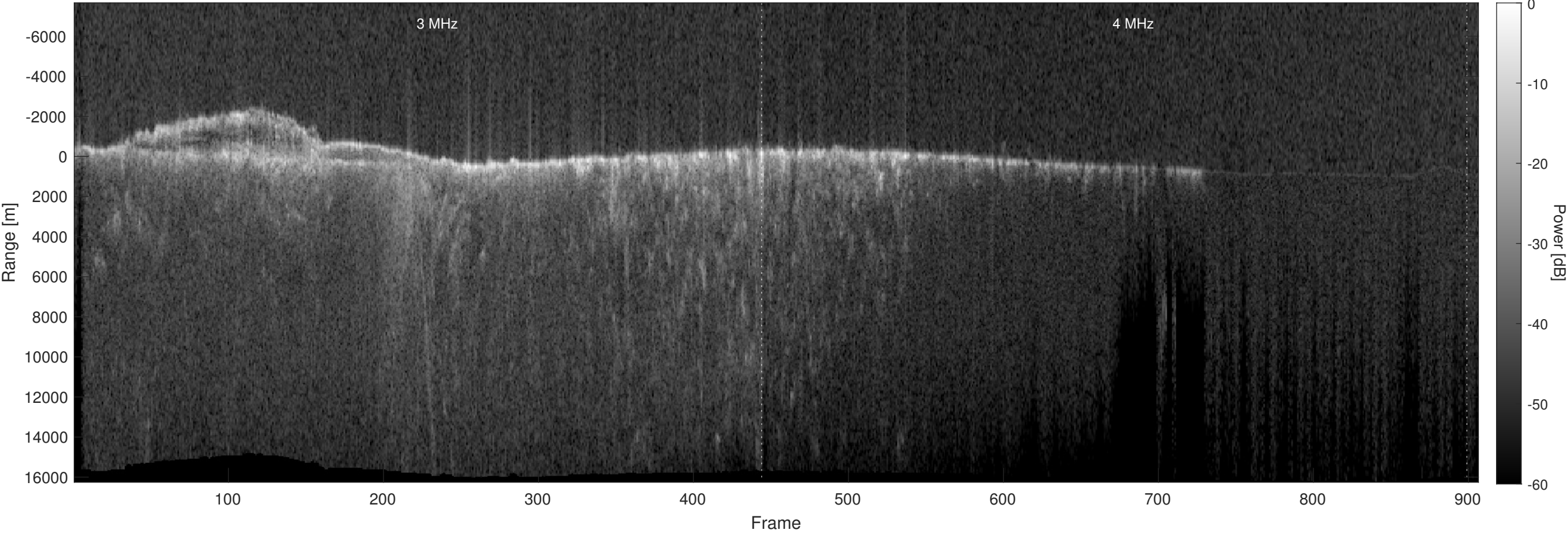
Orbit 11651, Optimized, Window, Depth-Corrected, Channel 2
