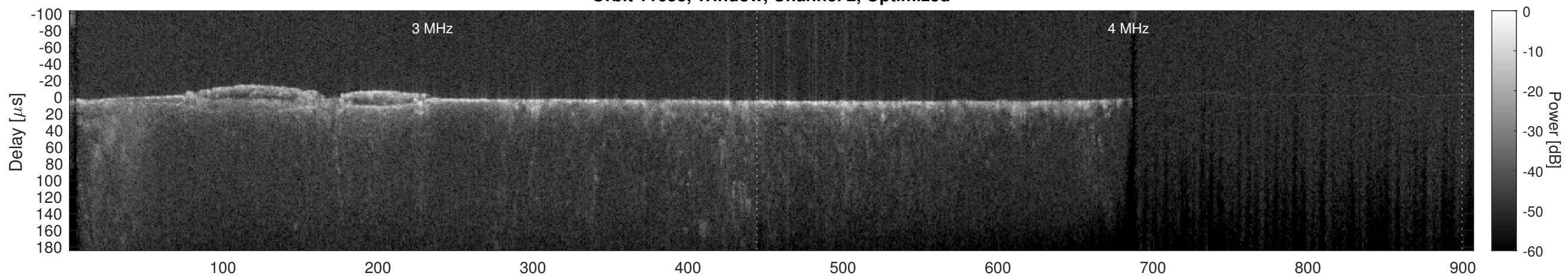
Orbit 11653, Cluttergram
