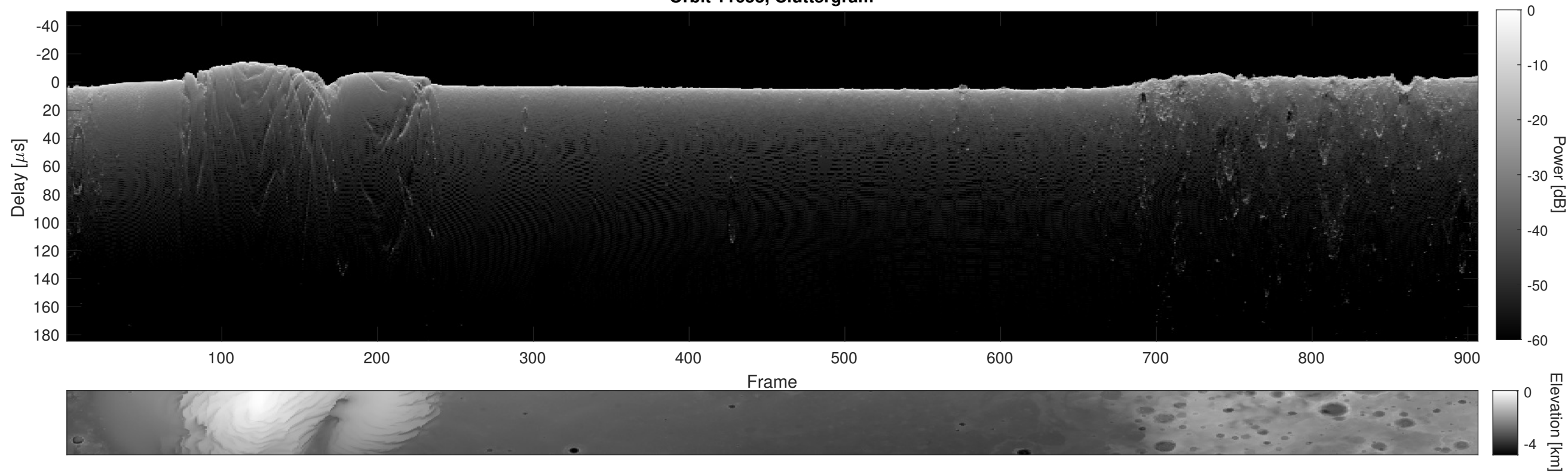
Orbit 11653, Cluttergram
