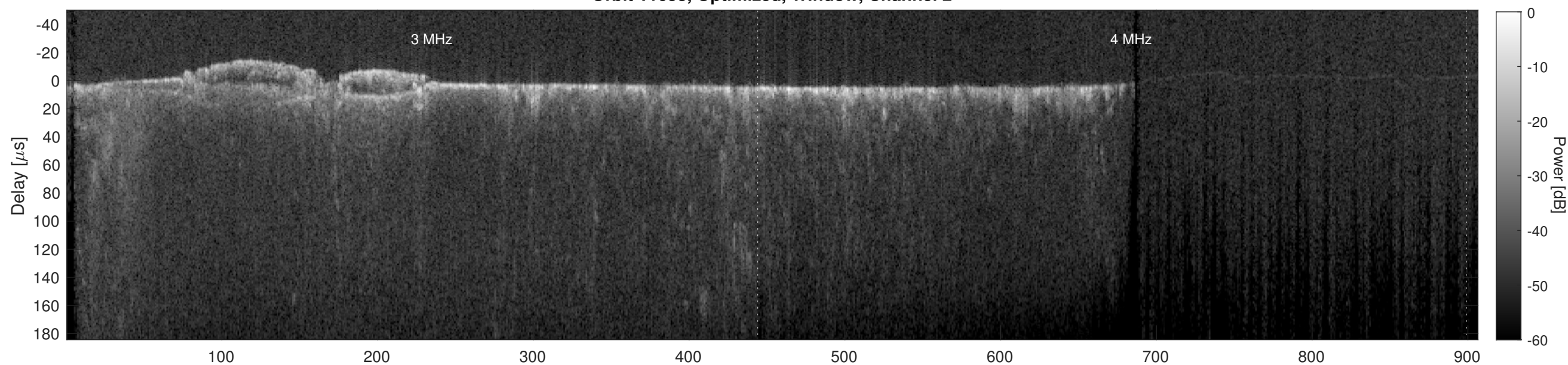
Orbit 11653, Cluttergram
