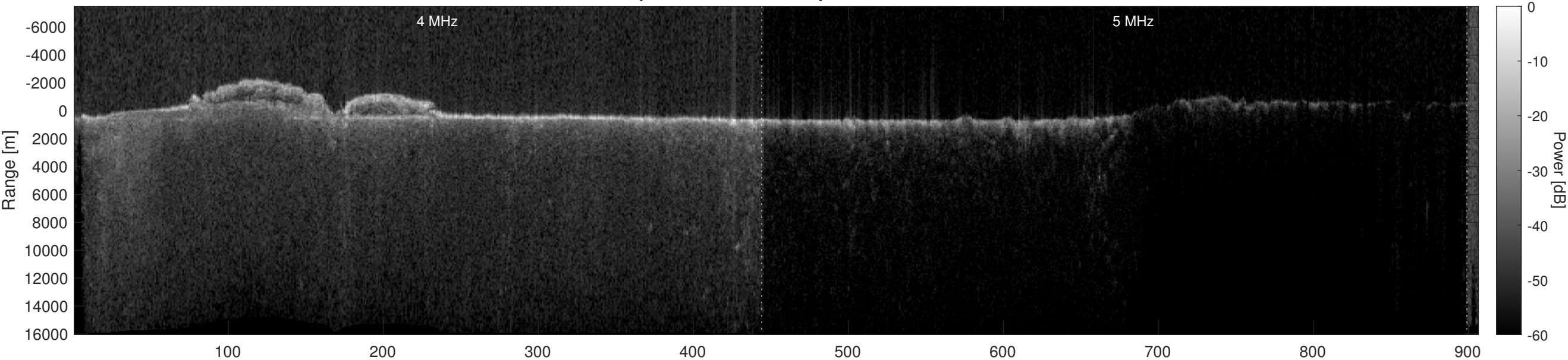
Orbit 11653, Optimized, Window, Depth-Corrected, Channel 2
