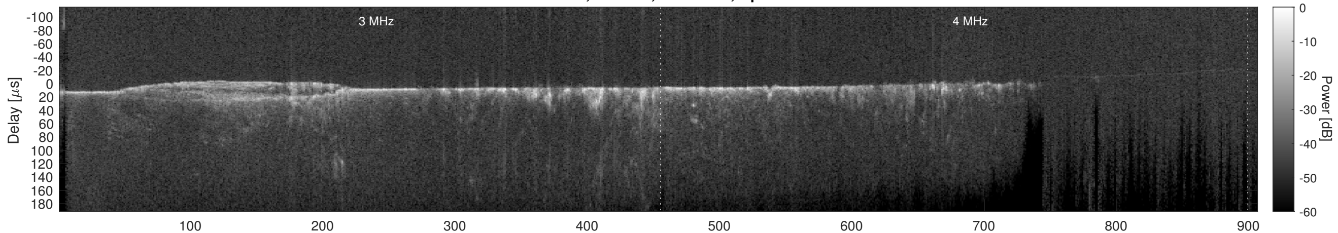
Orbit 11656, Cluttergram
