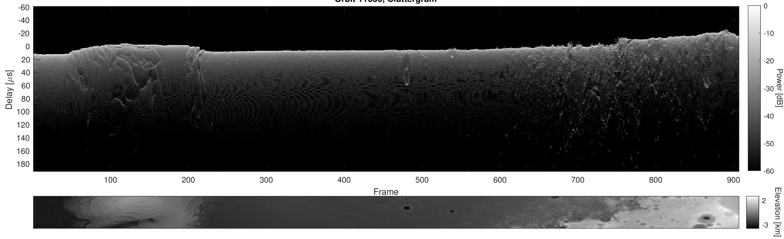
Orbit 11656, Cluttergram
