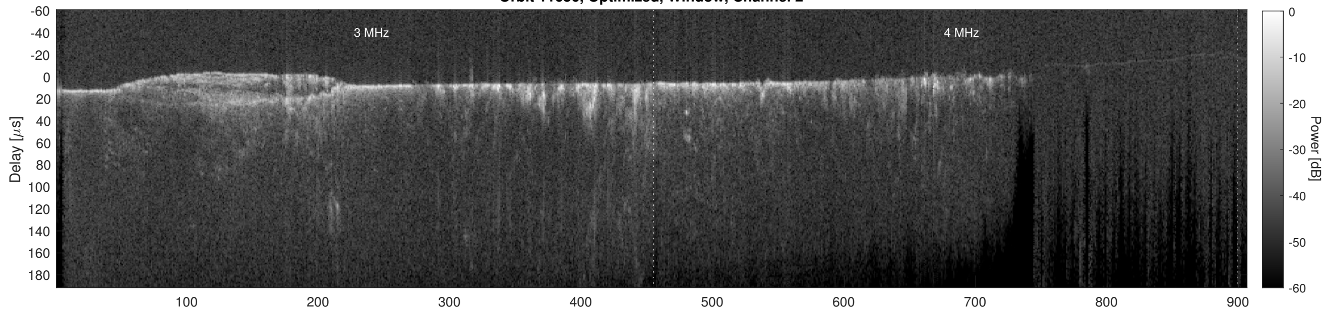
Orbit 11656, Cluttergram
