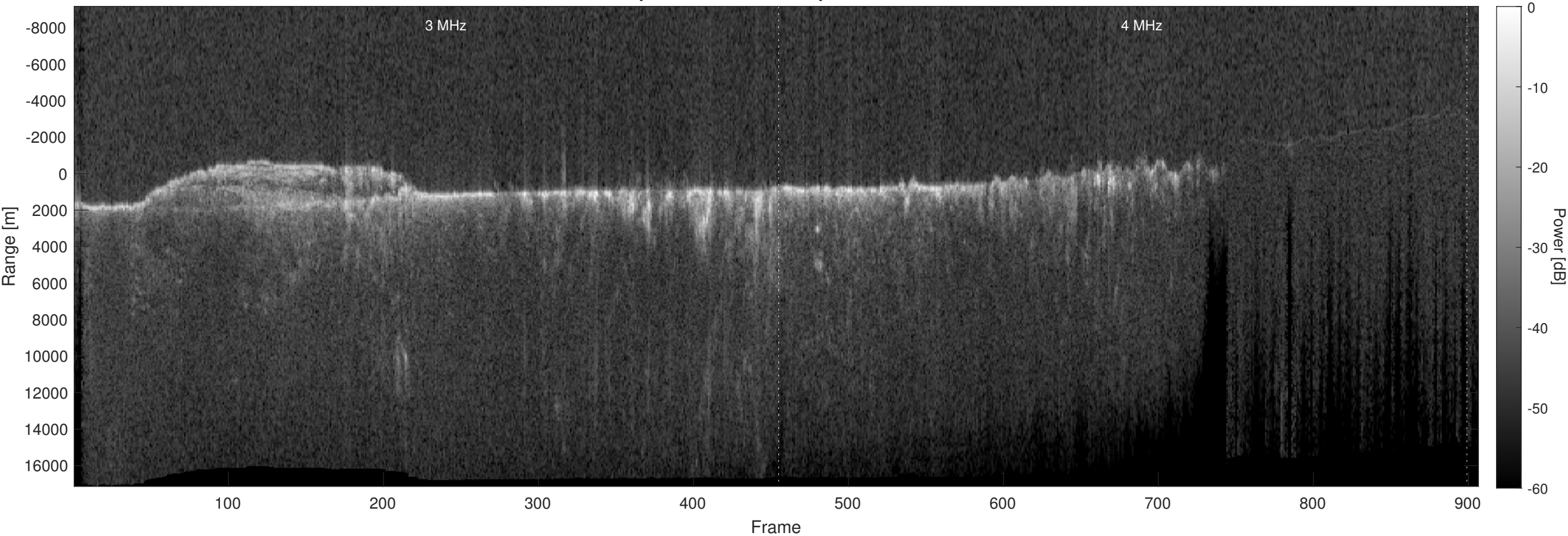
Orbit 11656, Optimized, Window, Depth-Corrected, Channel 2
