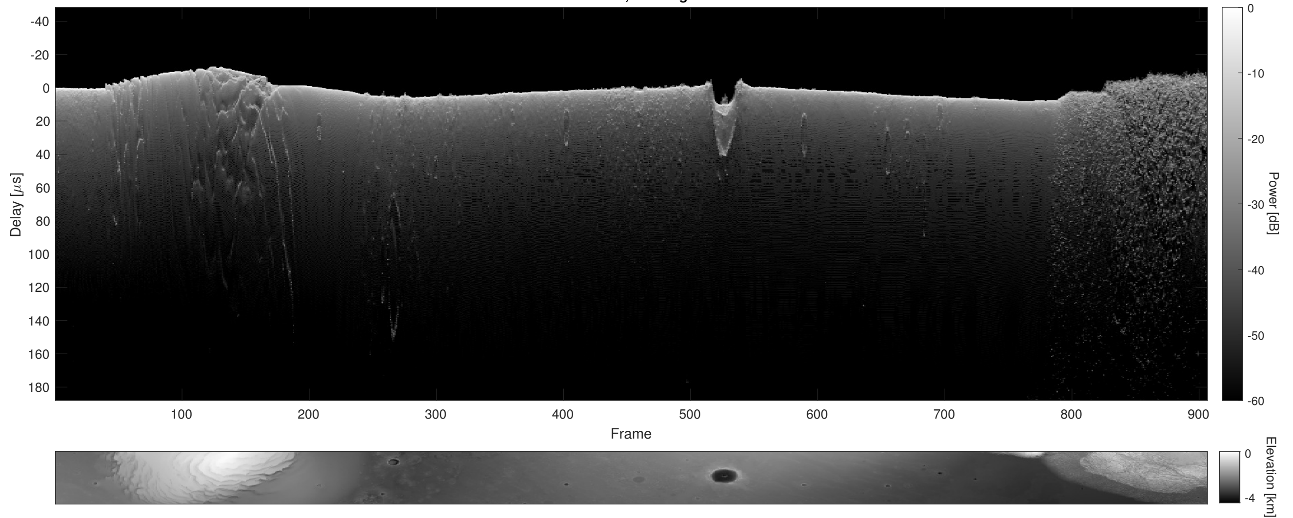
Orbit 11658, Cluttergram
