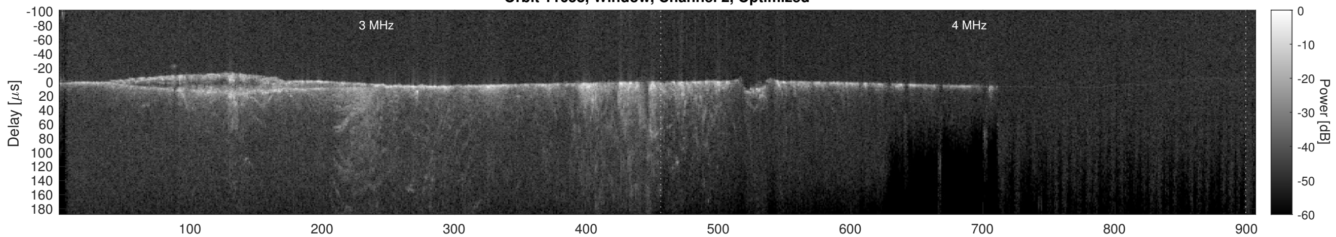
Orbit 11658, Cluttergram
