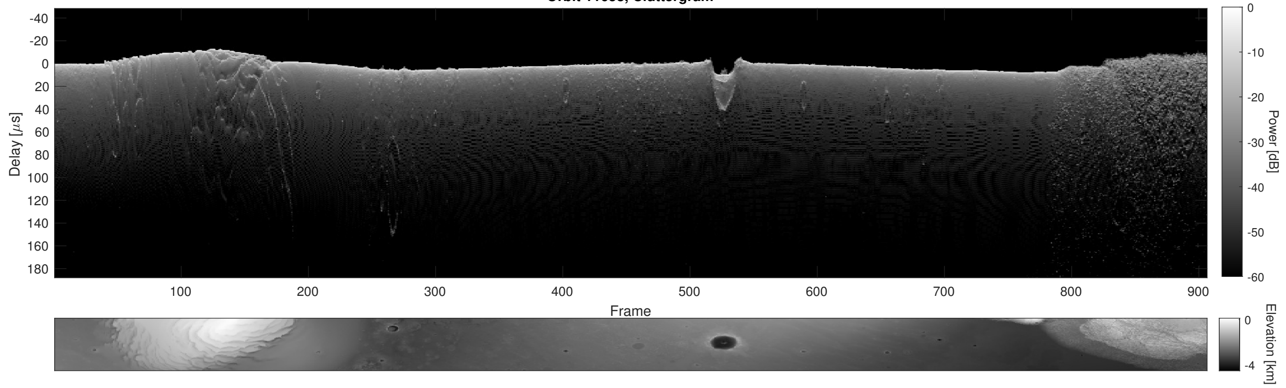
Orbit 11658, Cluttergram
