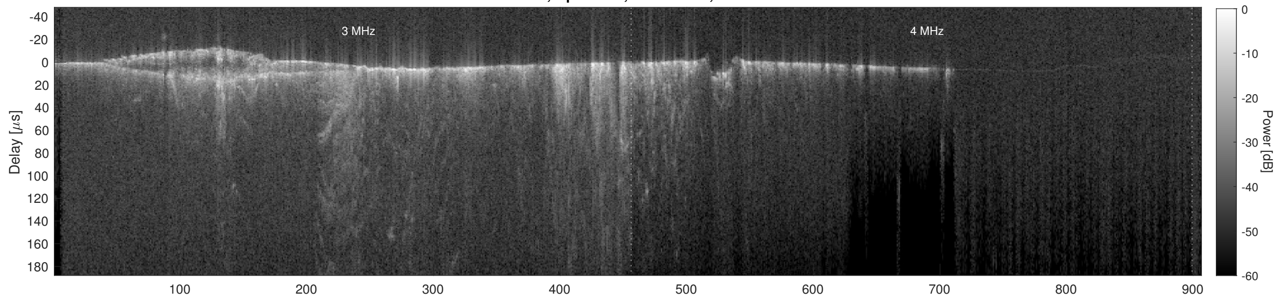
Orbit 11658, Cluttergram
