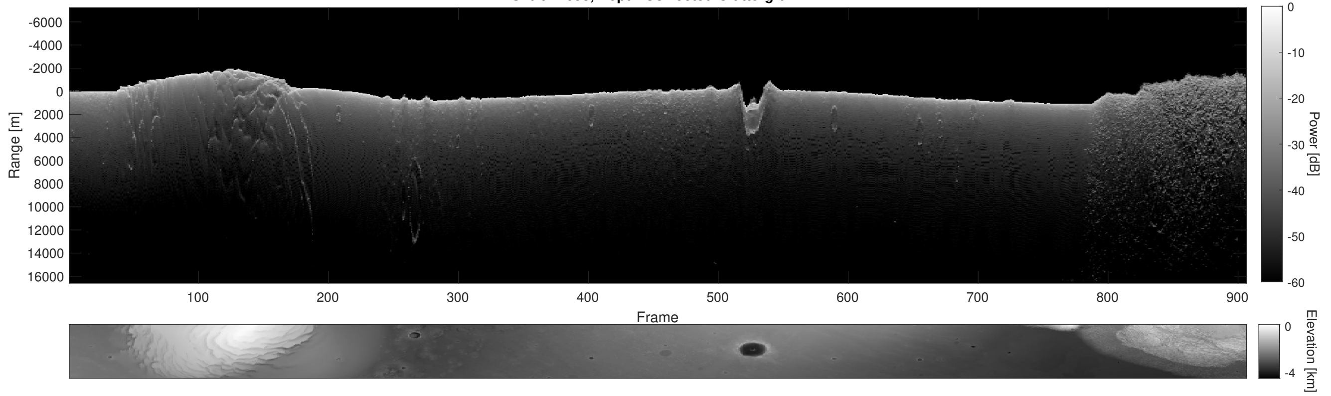
Orbit 11658, Depth-Corrected Cluttergram
