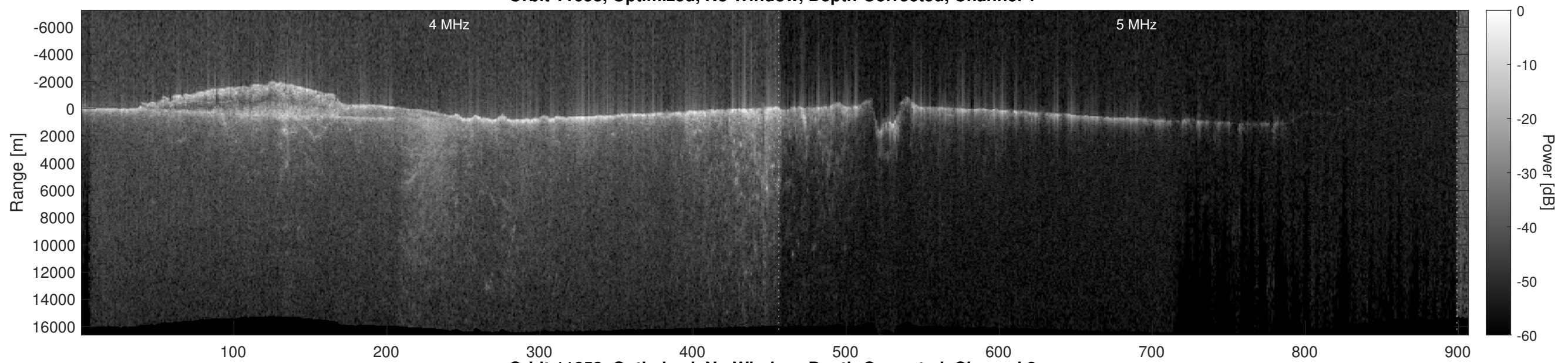
Orbit 11658, Optimized, No Window, Depth-Corrected, Channel 2
