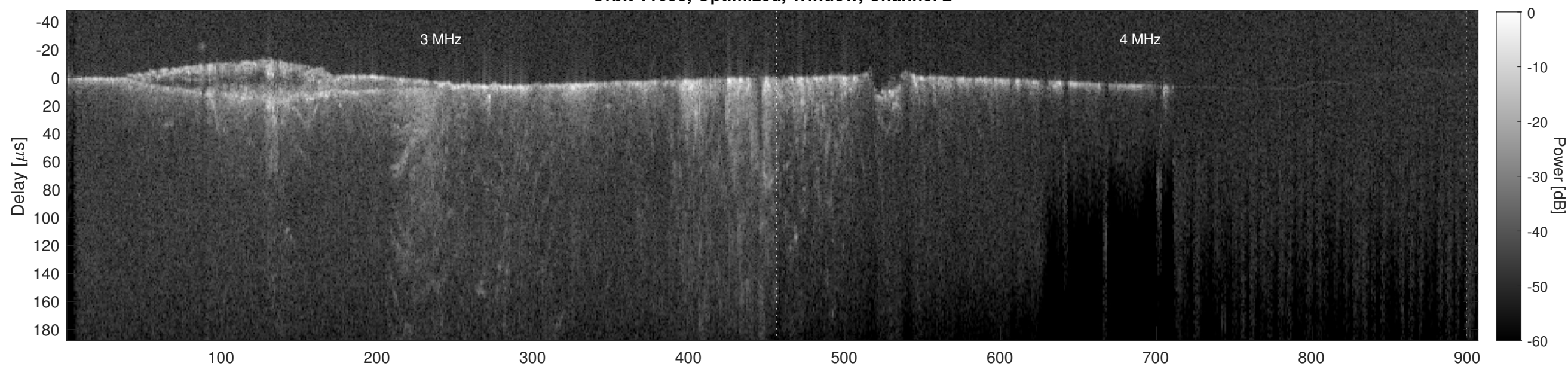
Orbit 11658, Cluttergram
