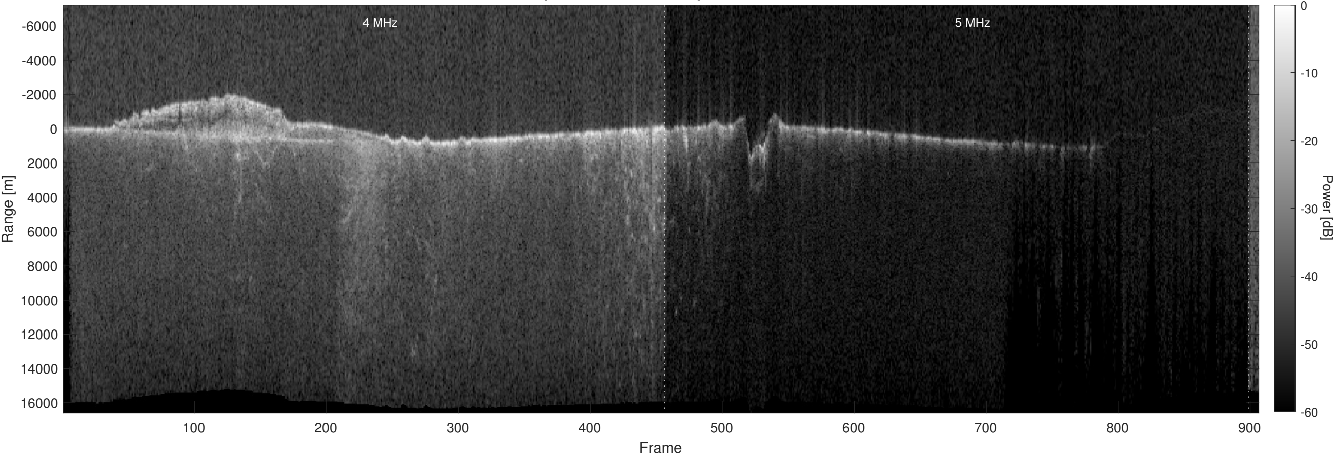
Orbit 11658, Optimized, Window, Depth-Corrected, Channel 2
