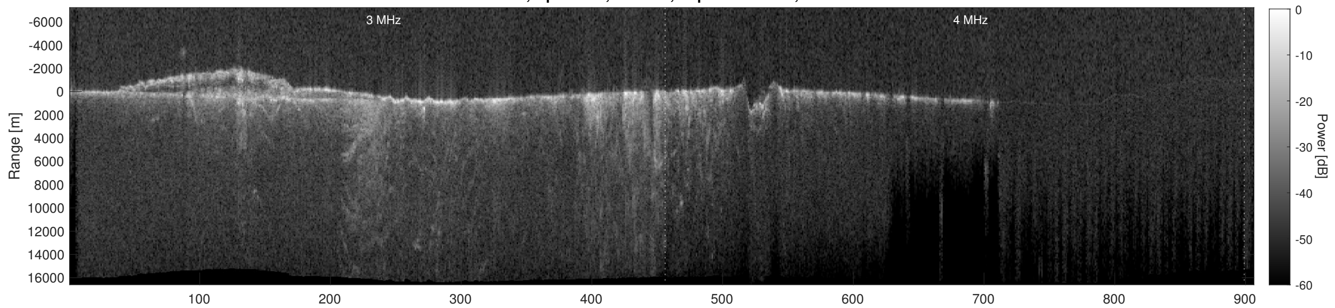
Orbit 11658, Depth-Corrected Cluttergram
