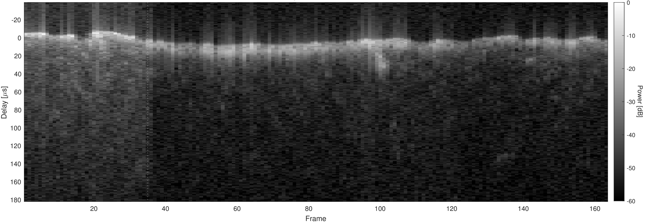
Orbit 11659, Chapman, No Window, Channel 2
