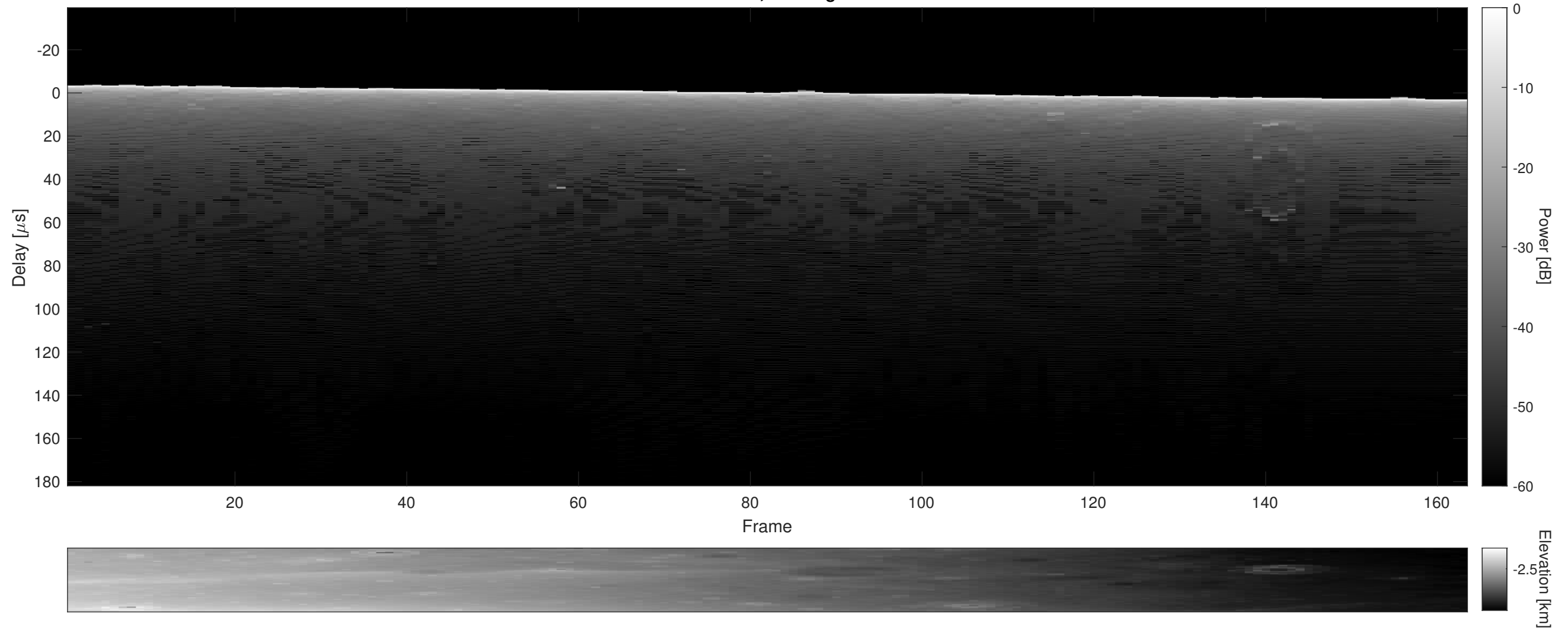
Orbit 11659, Cluttergram
