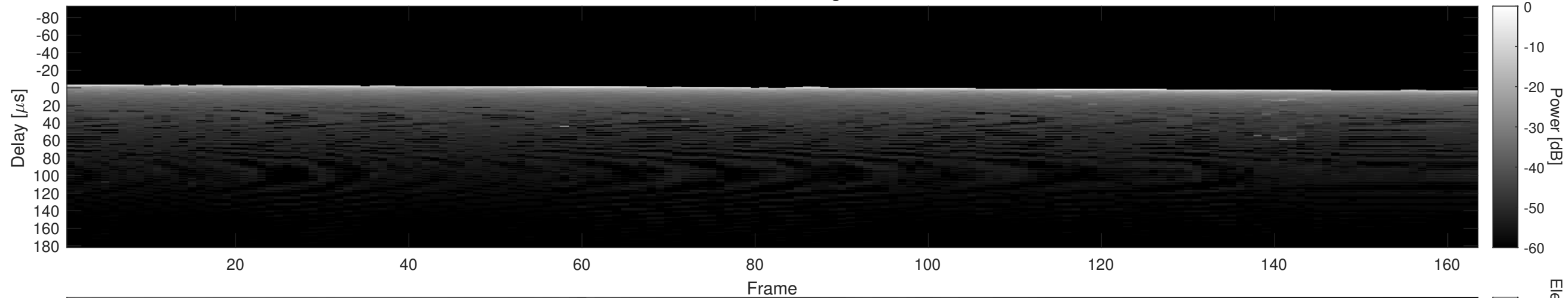
Orbit 11659, Cluttergram
