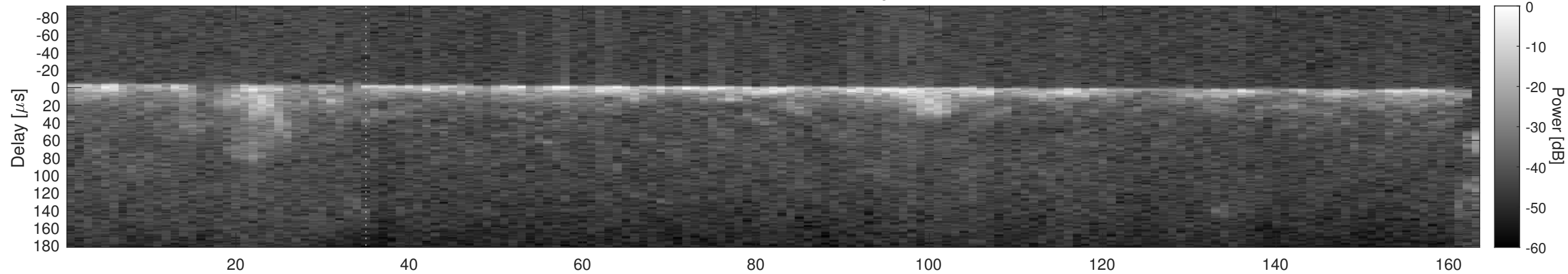
Orbit 11659, Cluttergram
