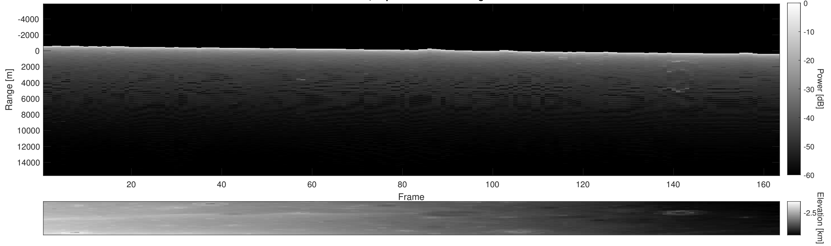
Orbit 11659, Depth-Corrected Cluttergram
