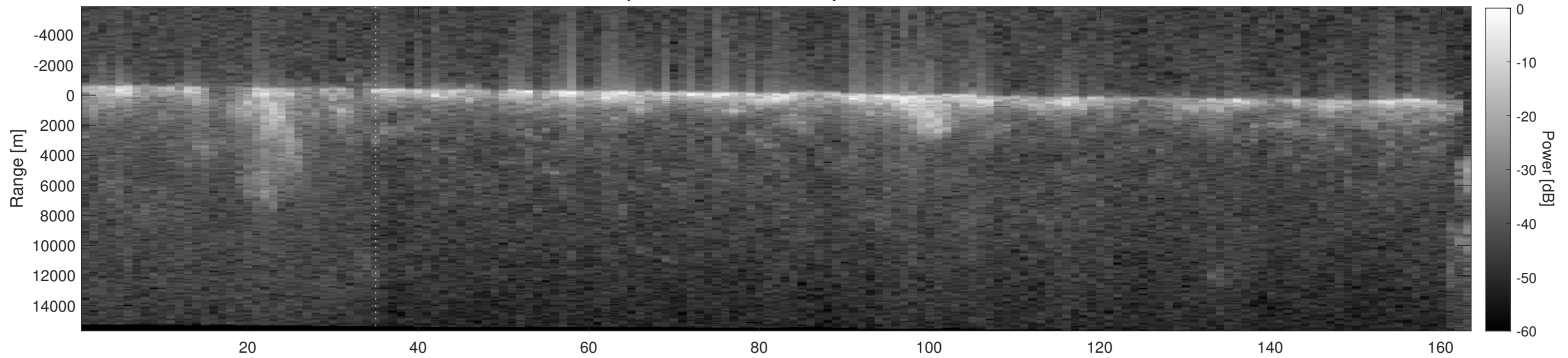
Orbit 11659, Depth-Corrected Cluttergram
