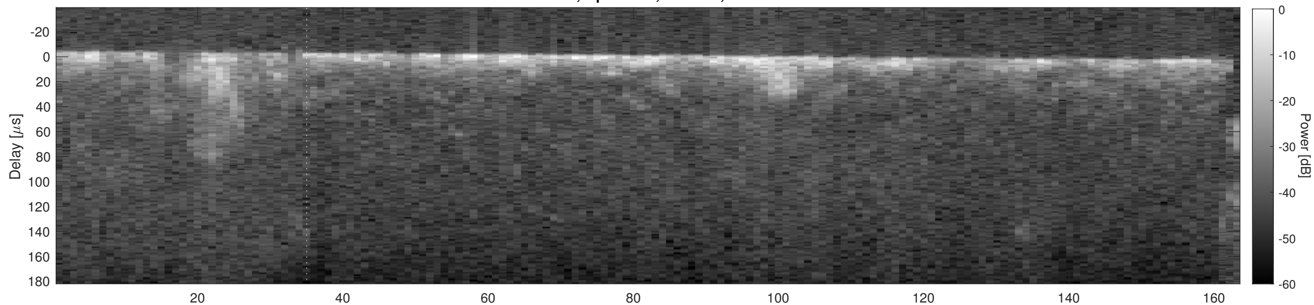
Orbit 11659, Cluttergram
