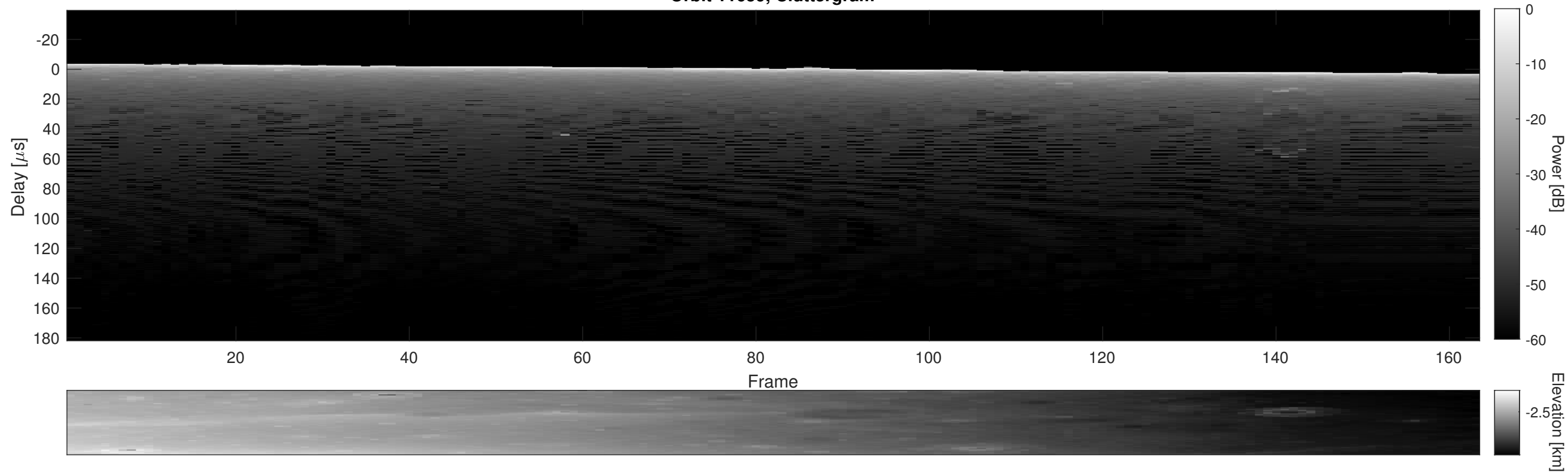
Orbit 11659, Cluttergram
