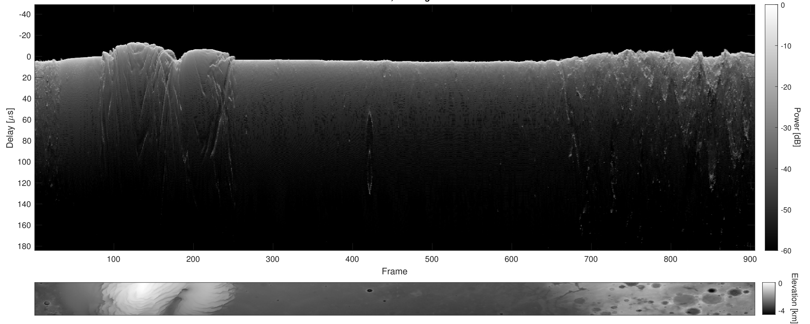
Orbit 11660, Cluttergram
