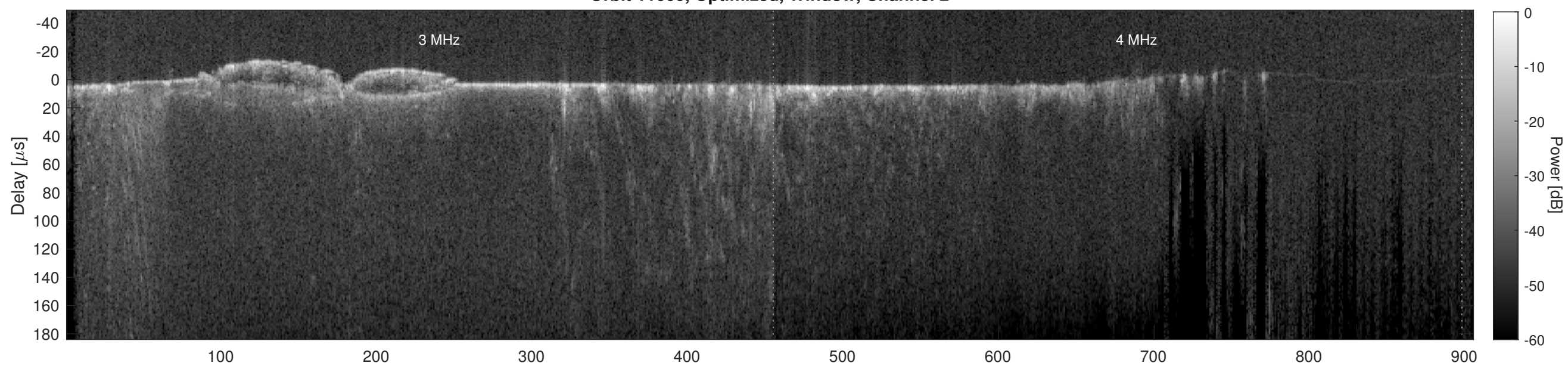
Orbit 11660, Cluttergram
