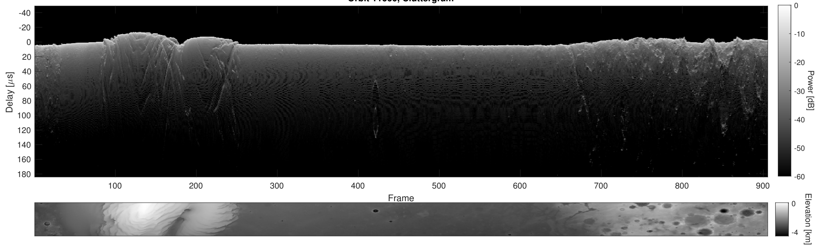
Orbit 11660, Cluttergram
