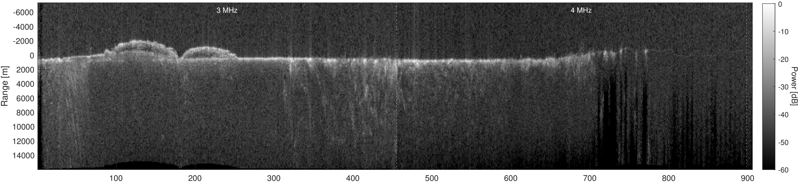
Orbit 11660, Depth-Corrected Cluttergram
