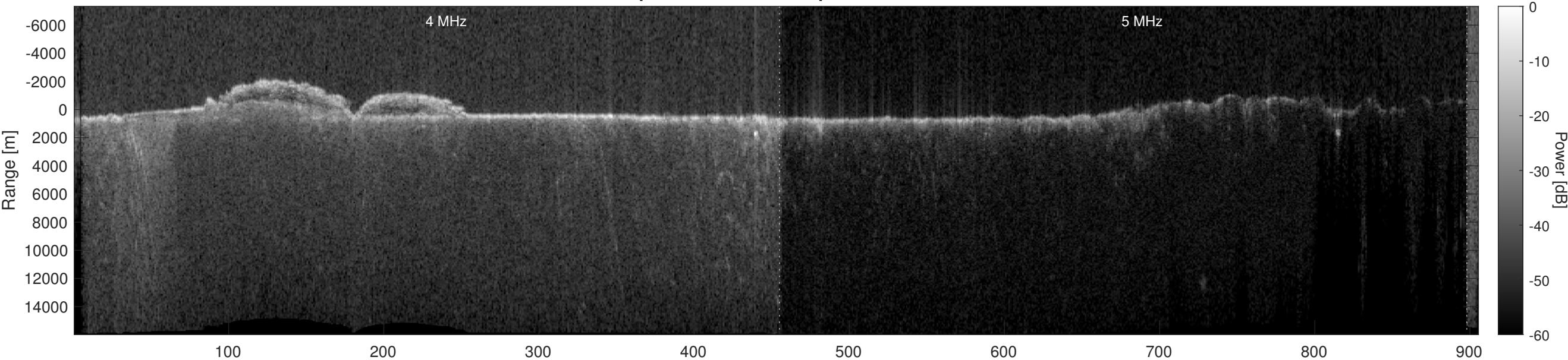
Orbit 11660, Optimized, Window, Depth-Corrected, Channel 2
