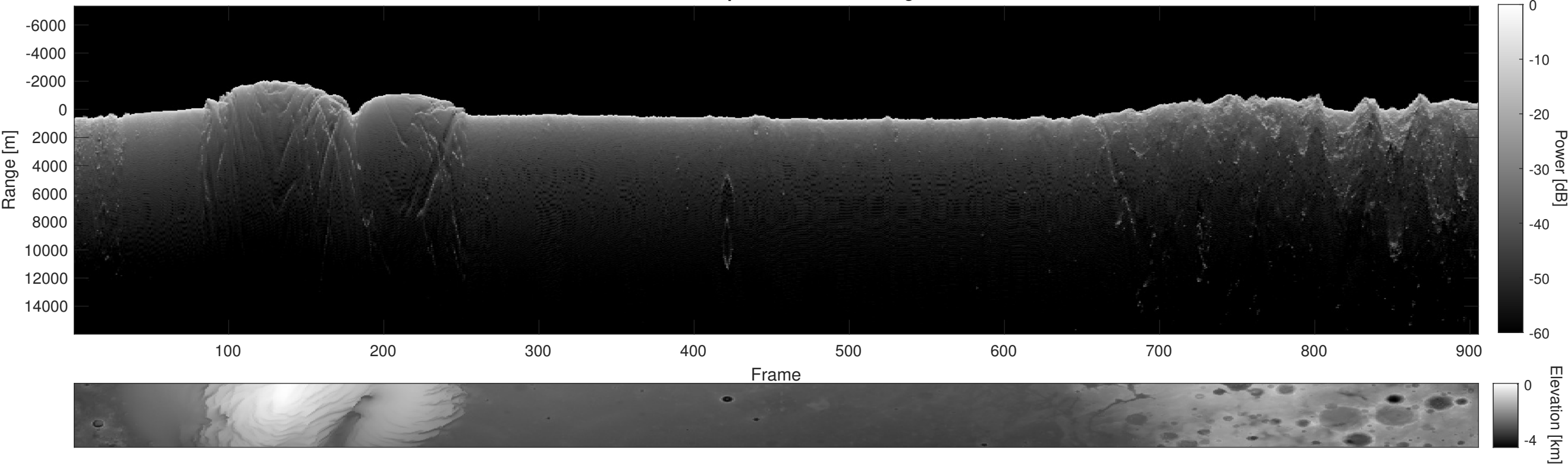
Orbit 11660, Depth-Corrected Cluttergram
