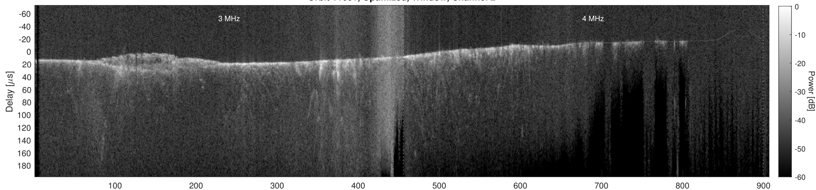
Orbit 11661, Cluttergram
