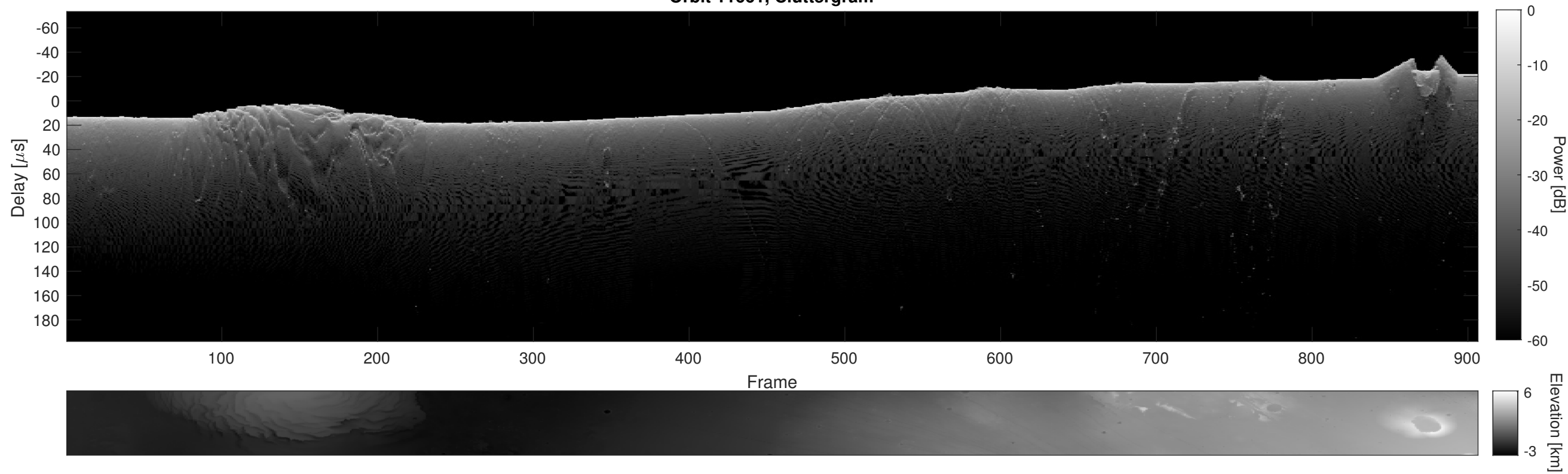
Orbit 11661, Cluttergram
