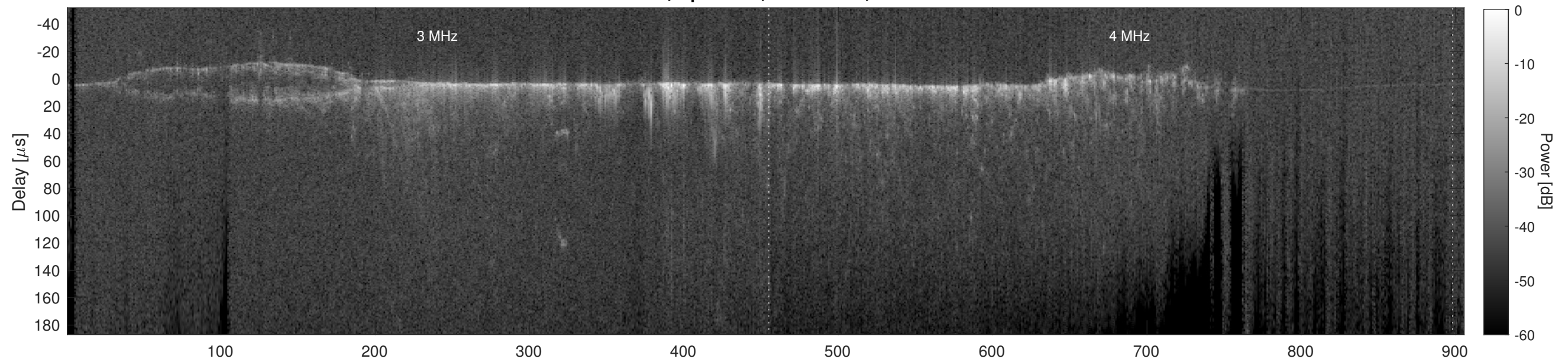
Orbit 11662, Cluttergram
