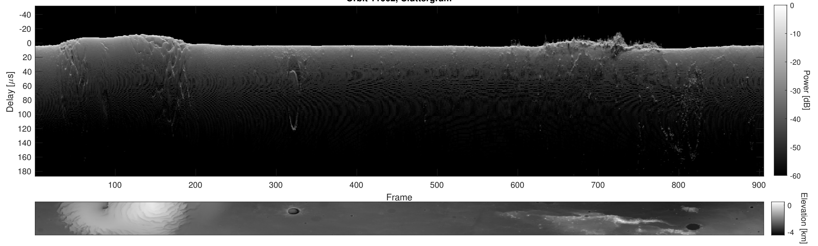
Orbit 11662, Cluttergram
