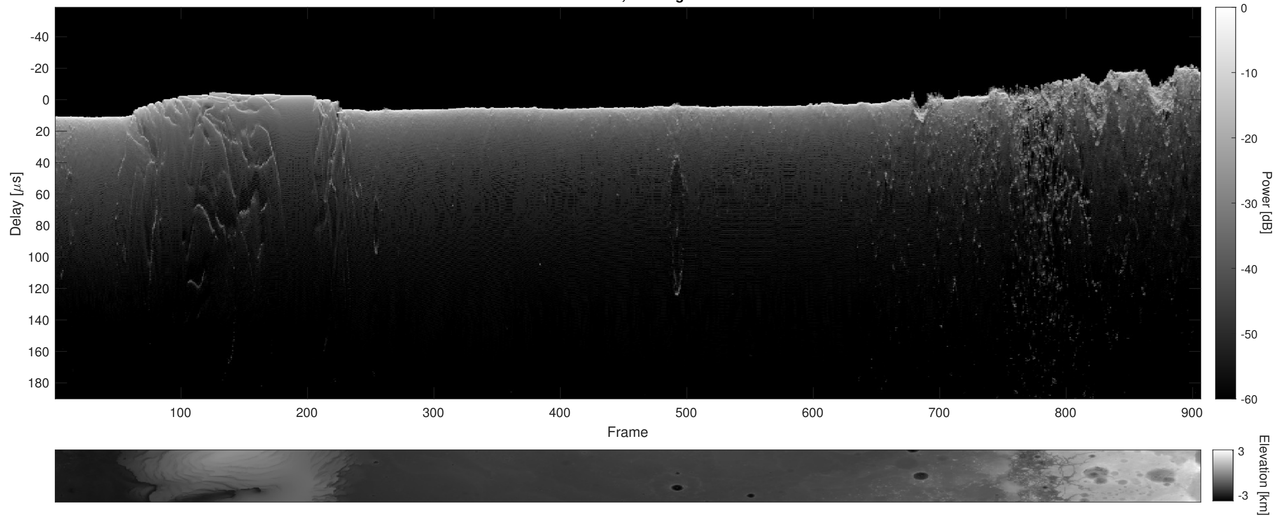
Orbit 11663, Cluttergram
