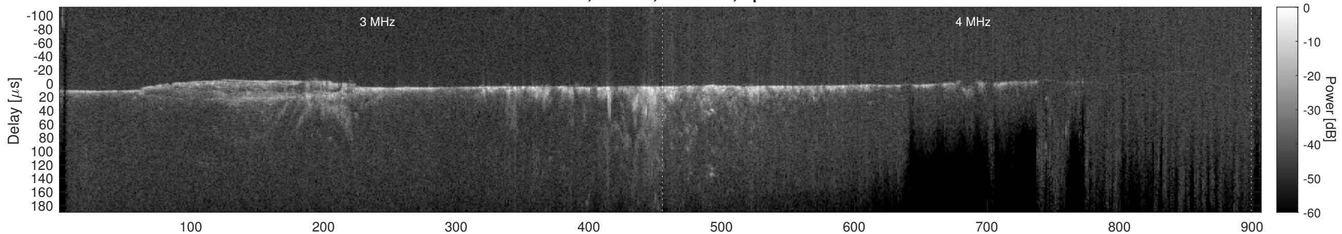
Orbit 11663, Cluttergram
