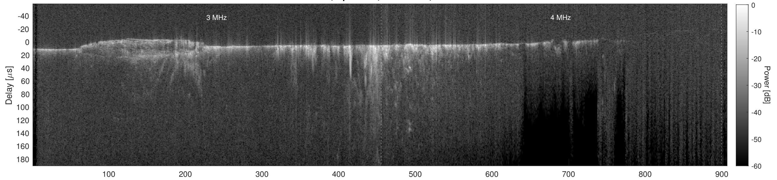
Orbit 11663, Cluttergram
