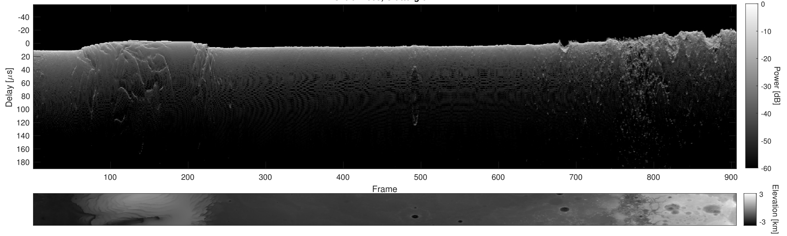
Orbit 11663, Cluttergram
