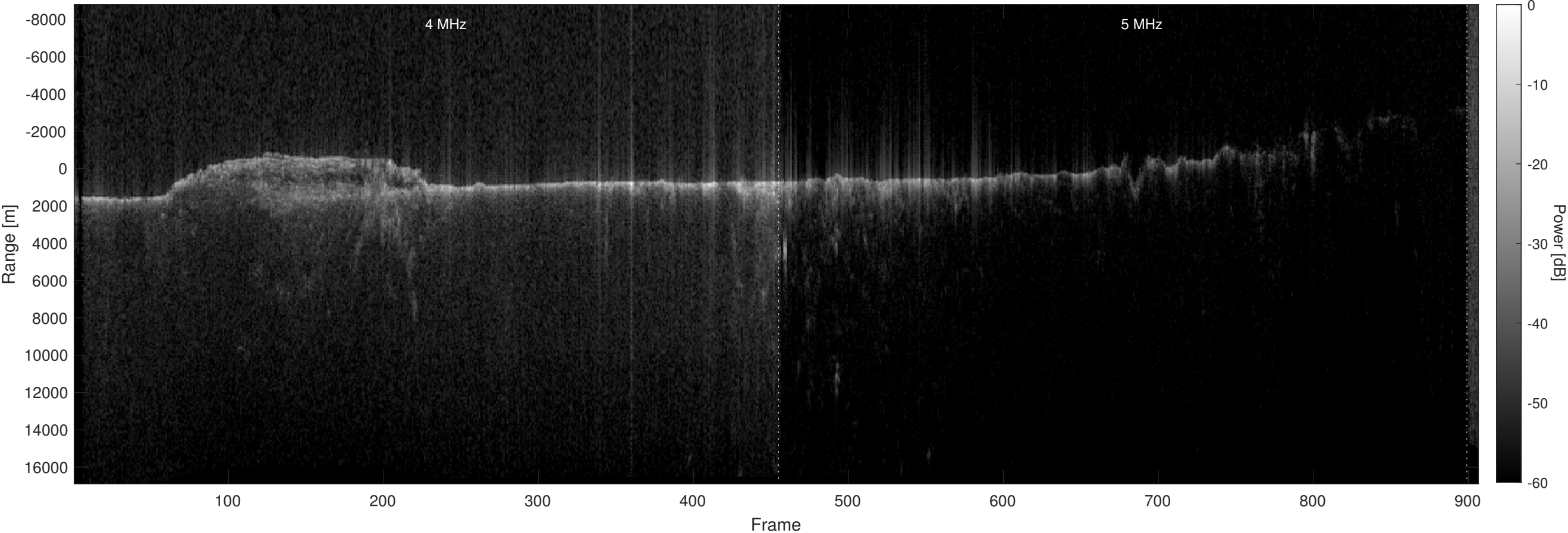
Orbit 11663, Optimized, No Window, Depth-Corrected, Channel 2
