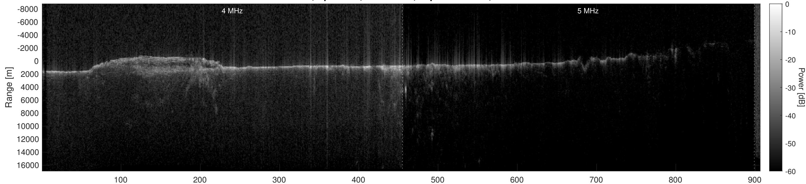
Orbit 11663, Optimized, No Window, Depth-Corrected, Channel 2
