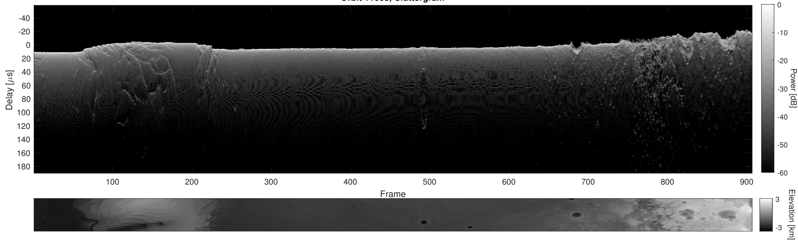
Orbit 11663, Cluttergram
