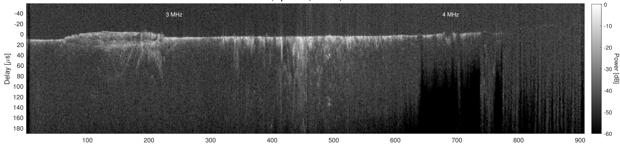
Orbit 11663, Cluttergram
