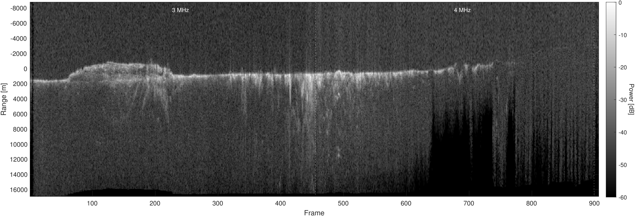
Orbit 11663, Optimized, Window, Depth-Corrected, Channel 2
