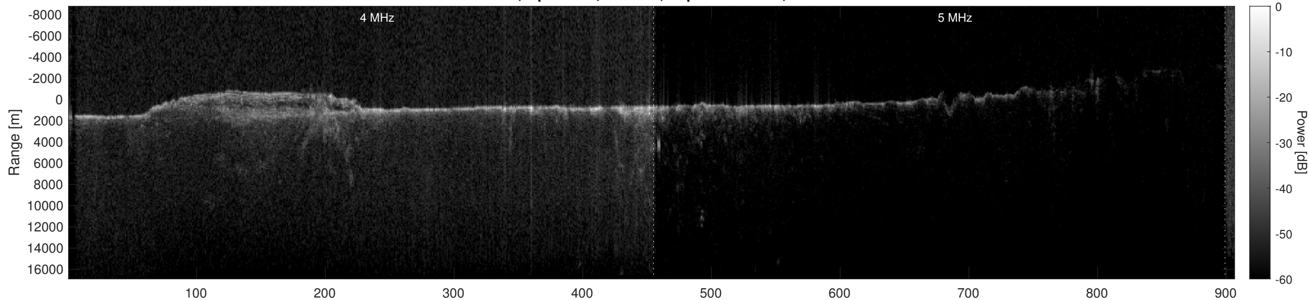
Orbit 11663, Optimized, Window, Depth-Corrected, Channel 2
