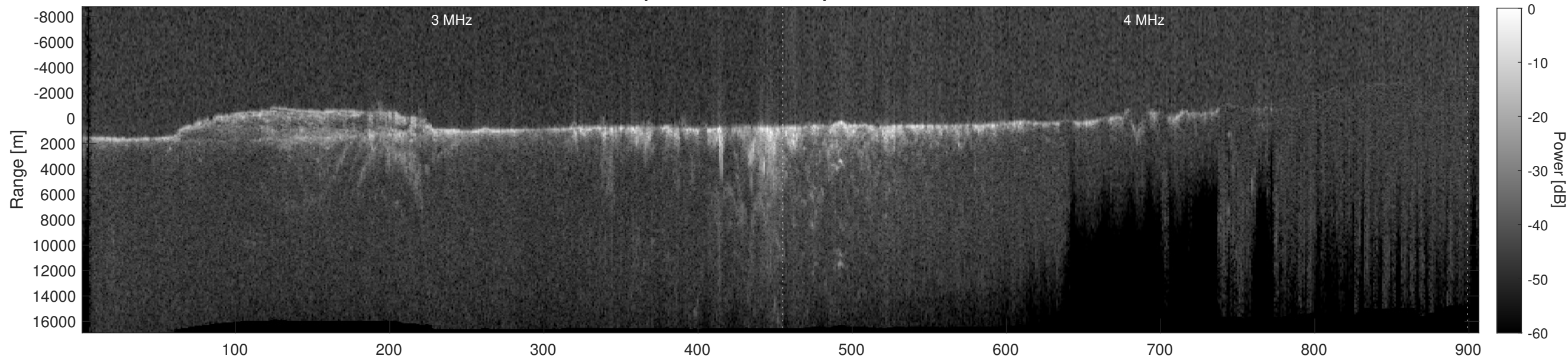
Orbit 11663, Depth-Corrected Cluttergram
