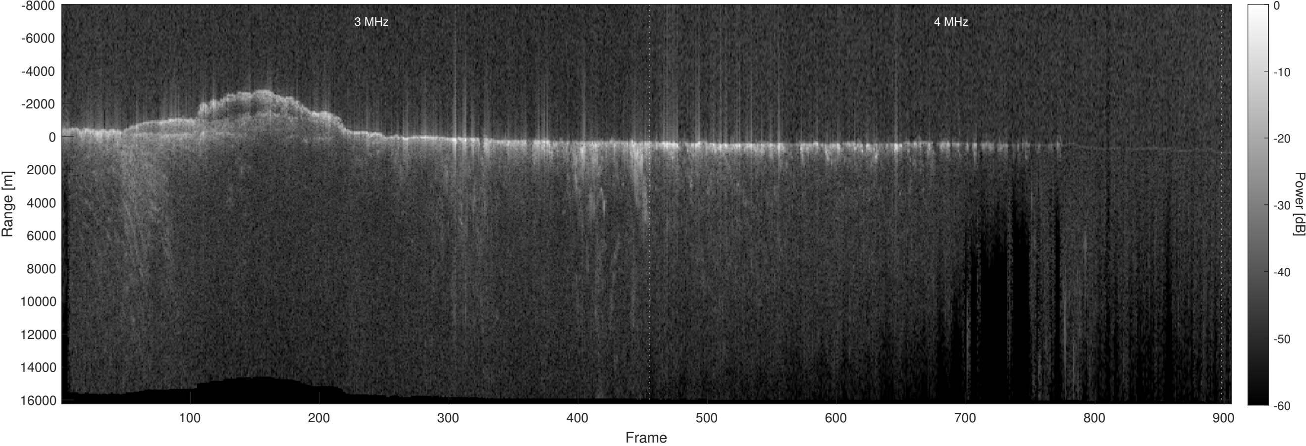
Orbit 11664, Optimized, No Window, Depth-Corrected, Channel 2
