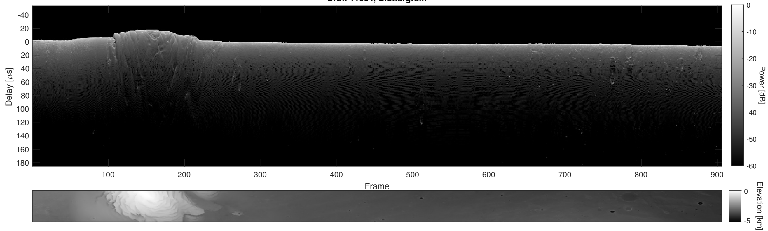
Orbit 11664, Cluttergram
