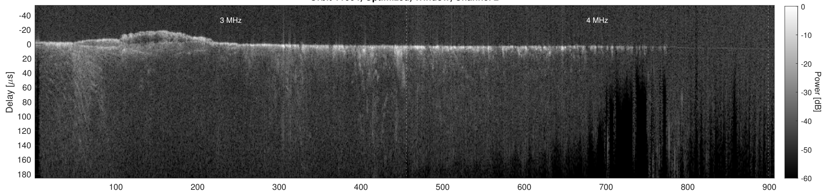
Orbit 11664, Cluttergram
