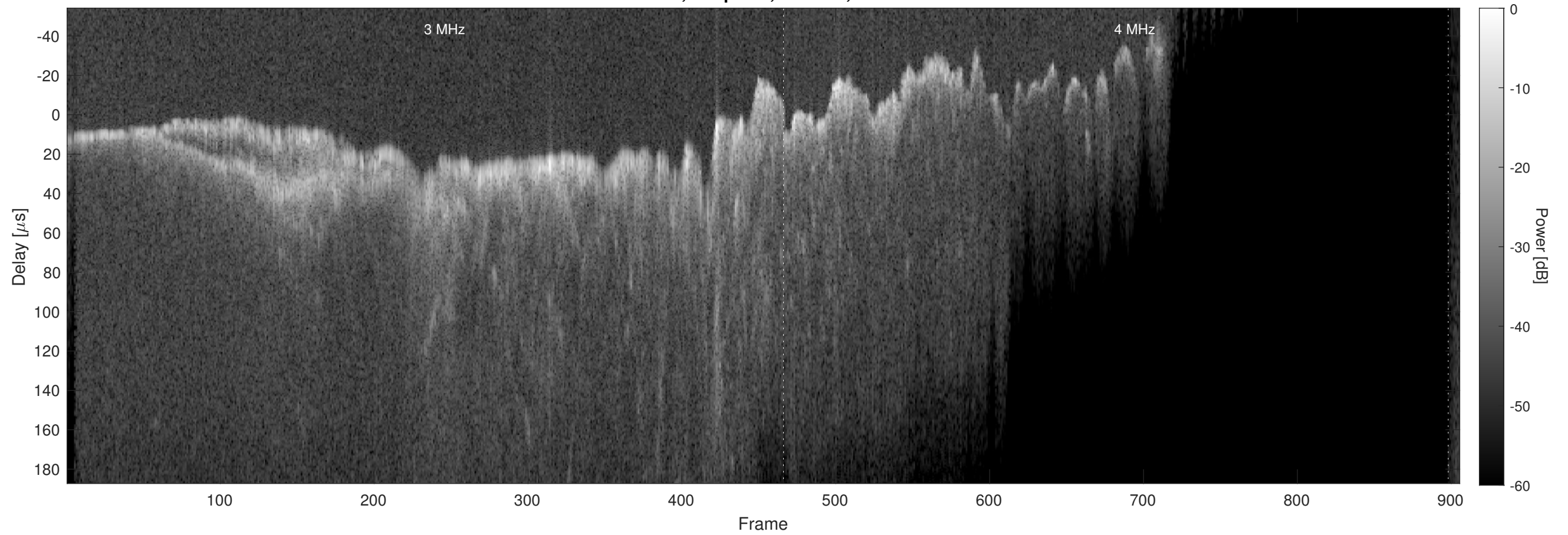
Orbit 11665, Chapman, Window, Channel 2
