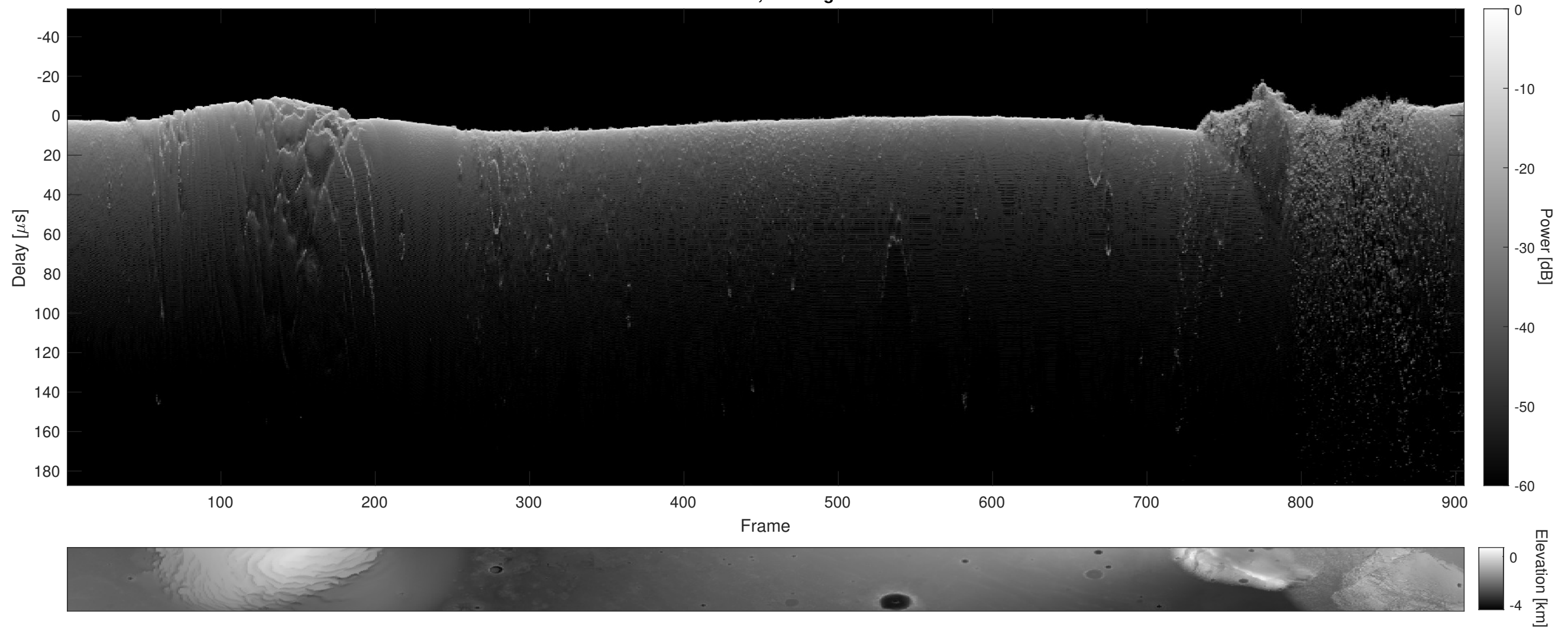
Orbit 11665, Cluttergram
