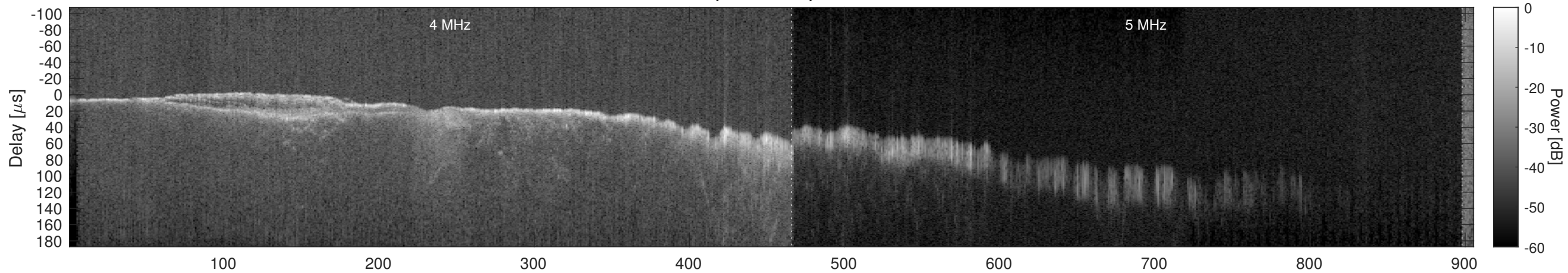
Orbit 11665, Window, Channel 1, Chapman
