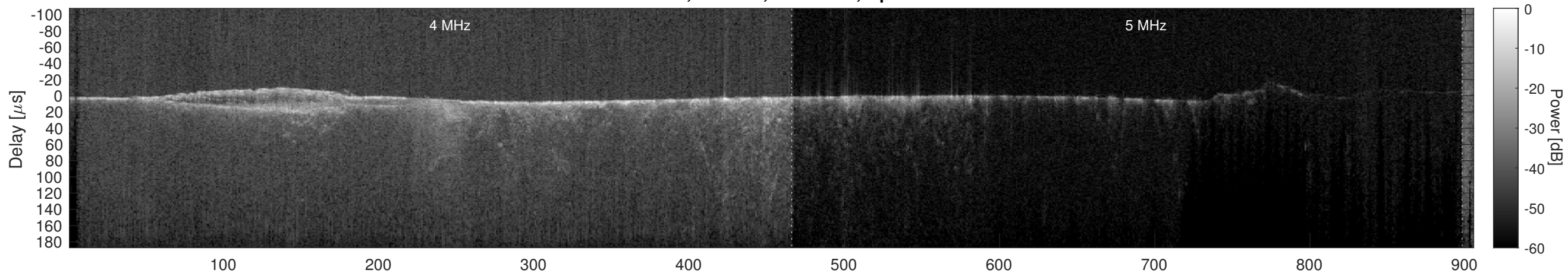
Orbit 11665, Cluttergram
