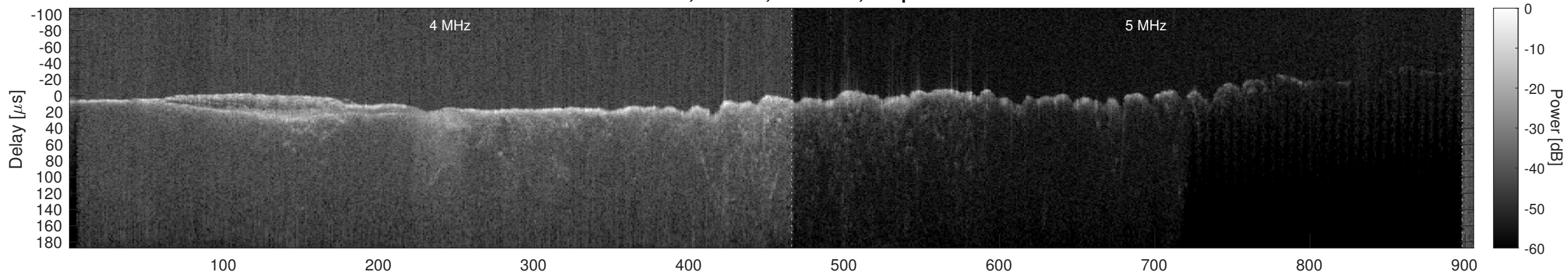
Orbit 11665, Window, Channel 1, Optimized
