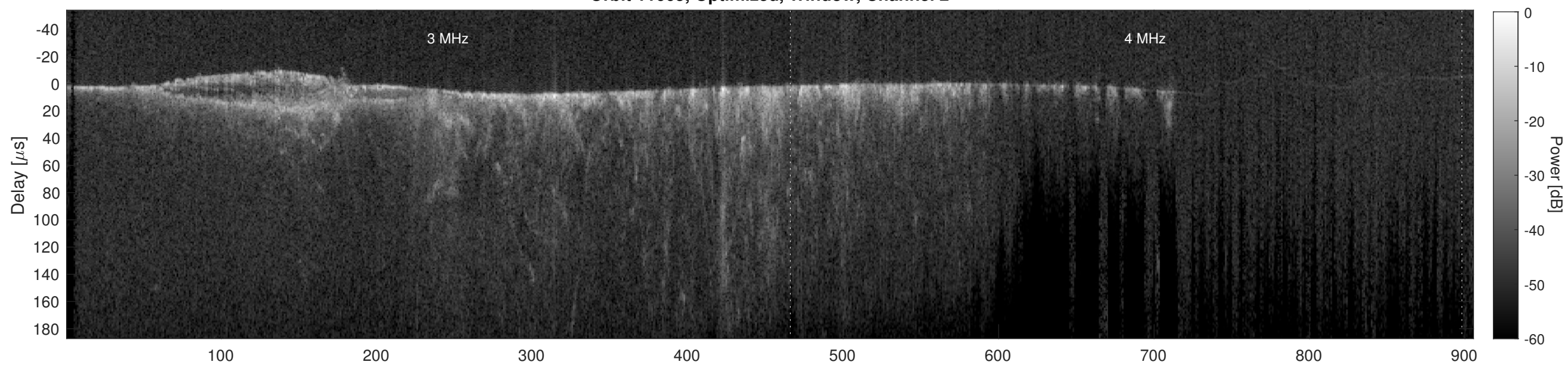
Orbit 11665, Cluttergram
