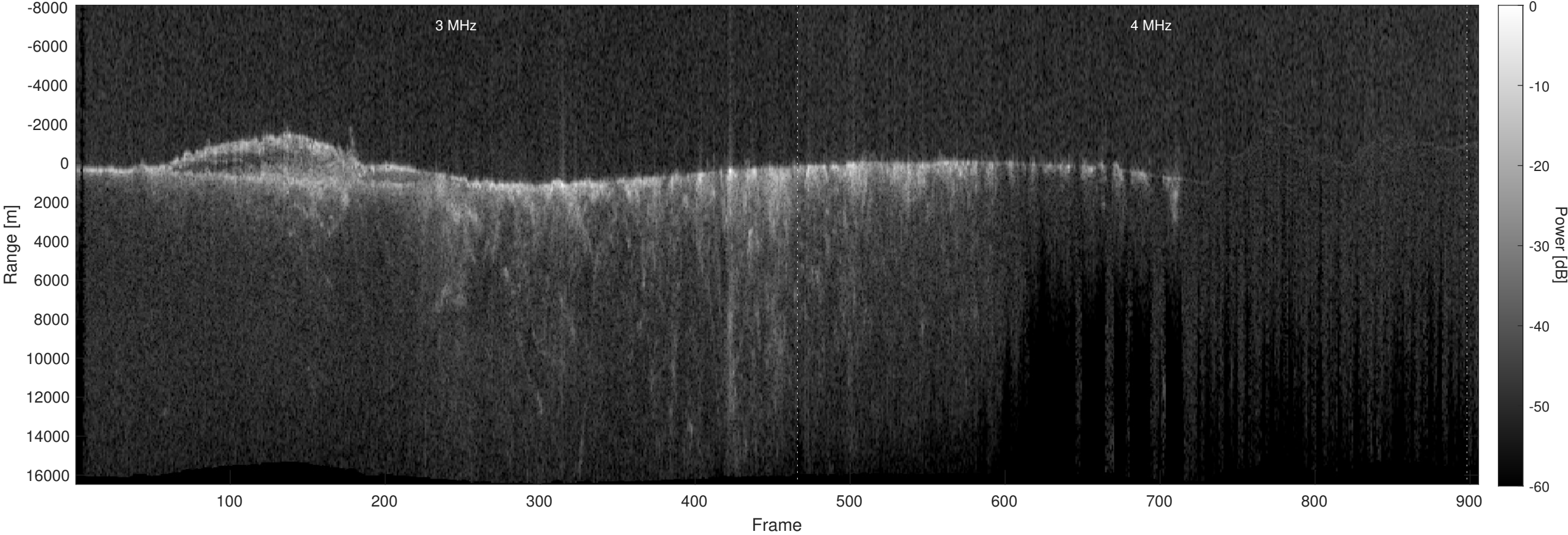
Orbit 11665, Optimized, Window, Depth-Corrected, Channel 2
