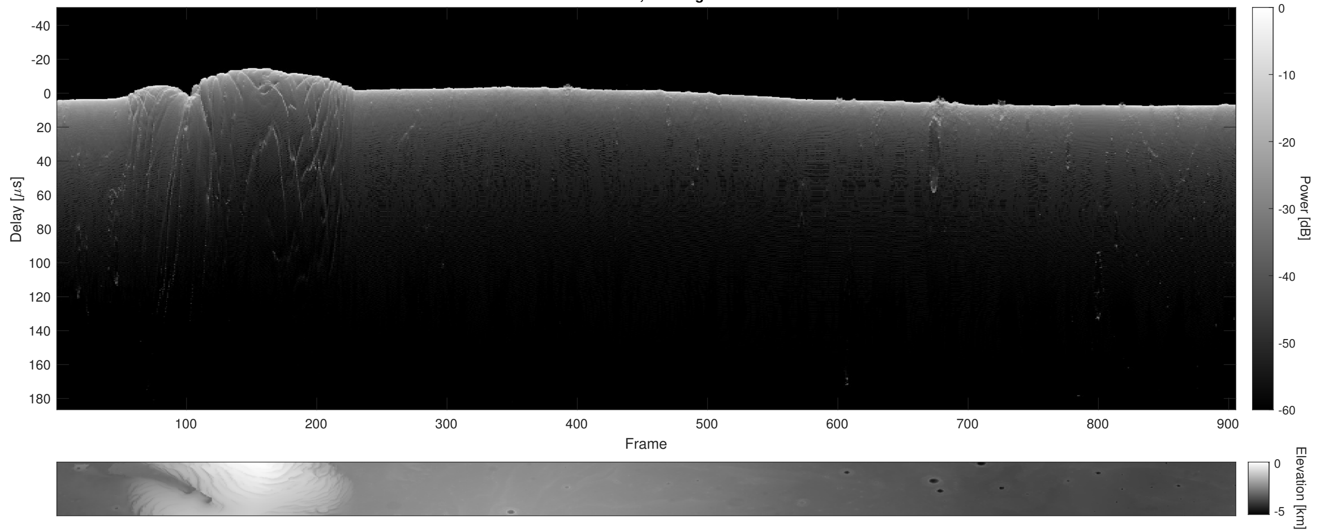
Orbit 11666, Cluttergram
