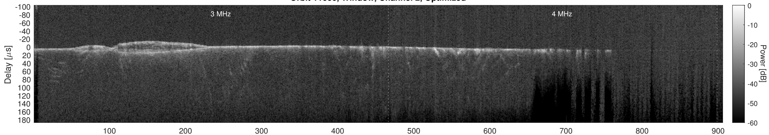
Orbit 11666, Cluttergram
