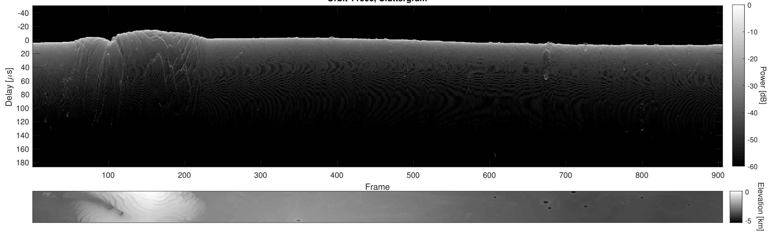
Orbit 11666, Cluttergram
