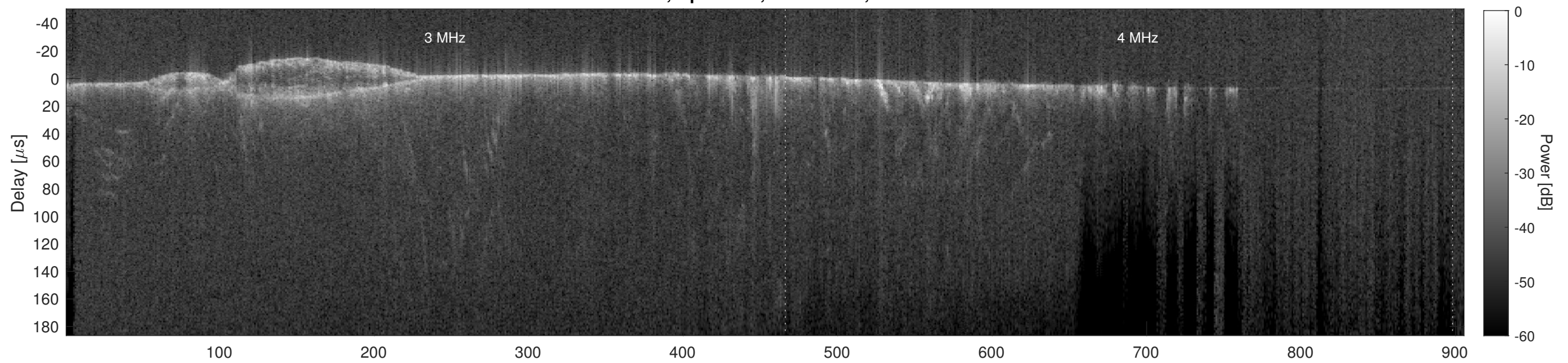
Orbit 11666, Cluttergram
