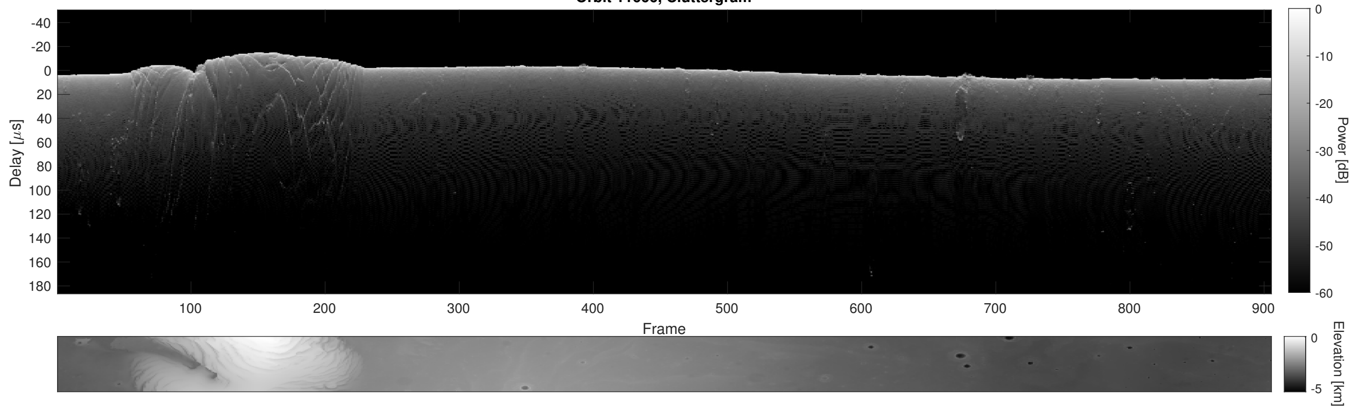
Orbit 11666, Cluttergram
