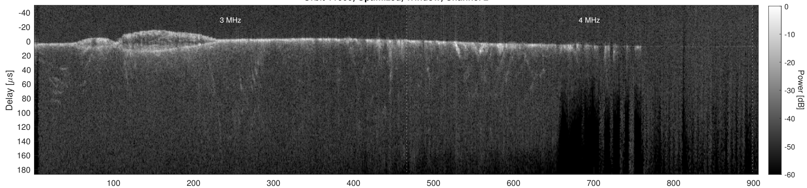
Orbit 11666, Cluttergram
