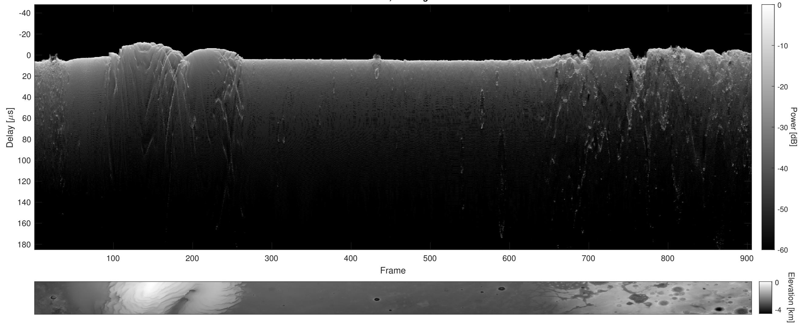
Orbit 11667, Cluttergram
