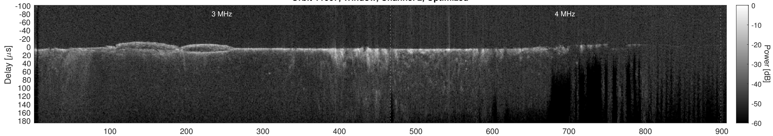
Orbit 11667, Cluttergram
