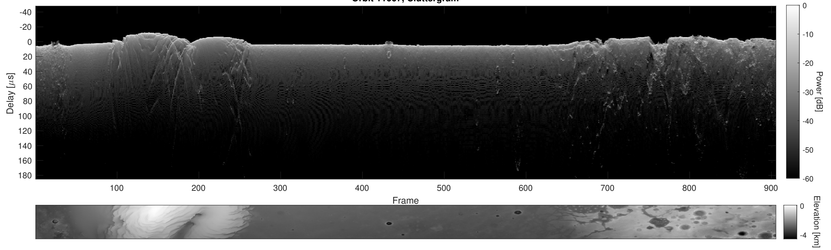
Orbit 11667, Cluttergram
