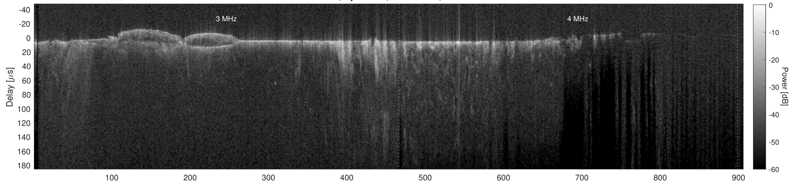
Orbit 11667, Cluttergram
