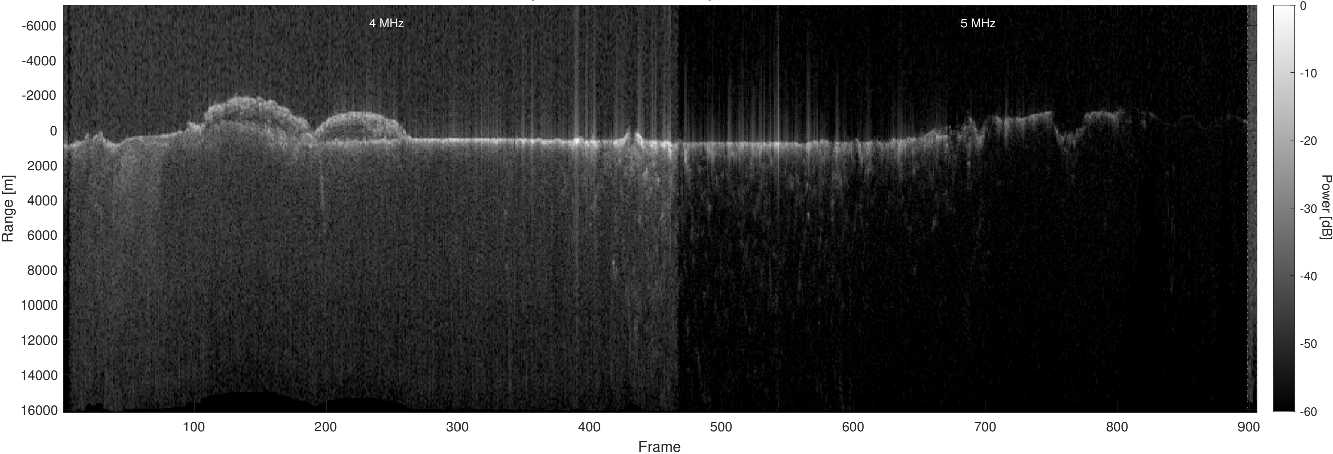
Orbit 11667, Optimized, No Window, Depth-Corrected, Channel 2
