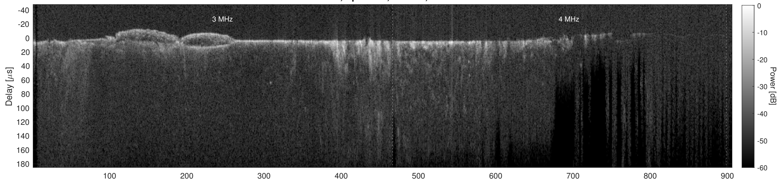
Orbit 11667, Cluttergram
