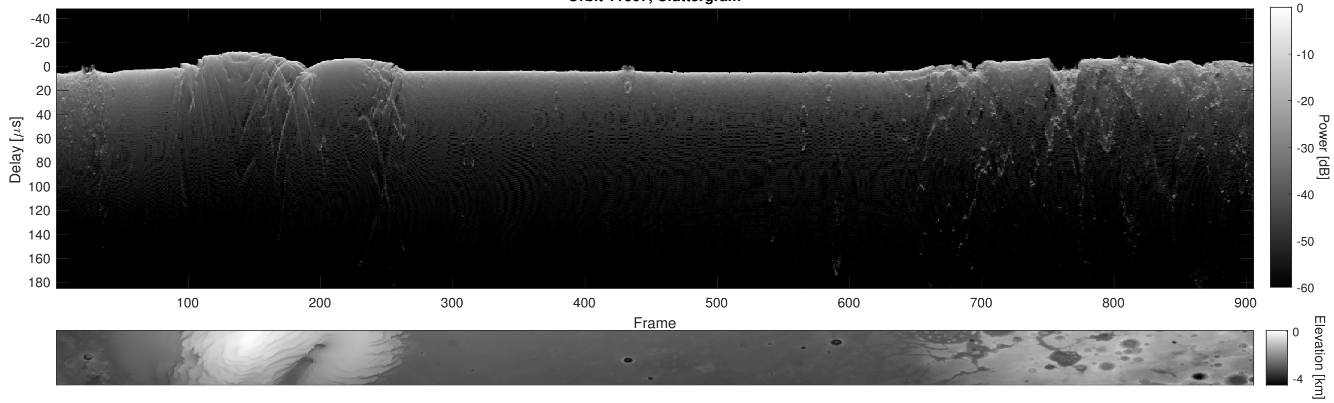
Orbit 11667, Cluttergram
